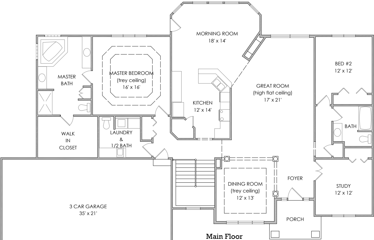
Main Floor
